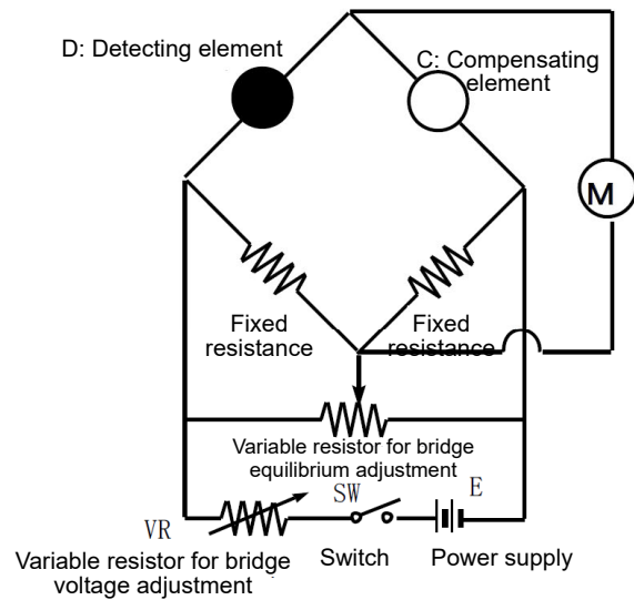
Basic Circuit
