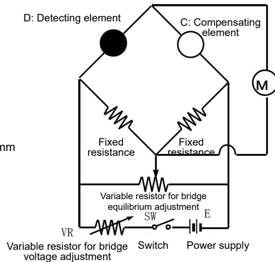
Basic Circuit
