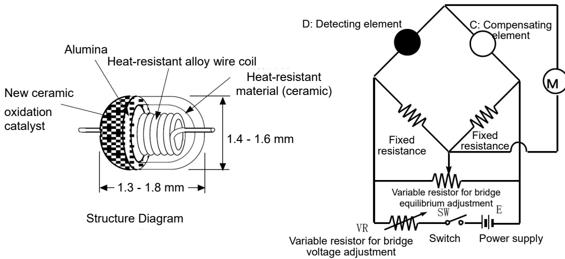
Basic Circuit
