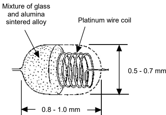
Structure Diagram
