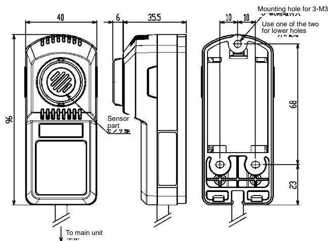
Remote sensor
