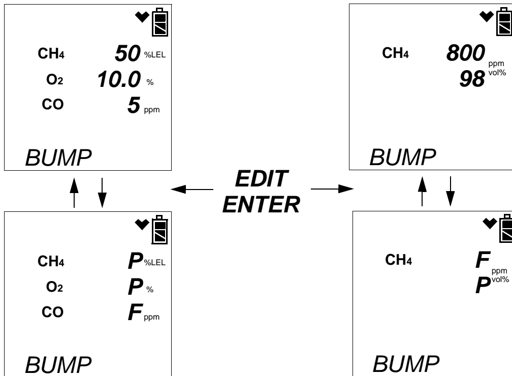
Figure 36: Failed Bump Test, AUTO CAL OFF, %Volume Sensor Installed and GAS Menu Item in Edit Mode Set to ALL
