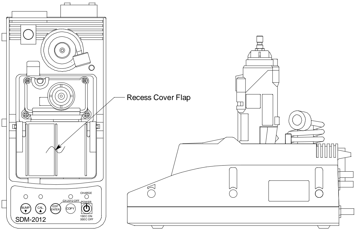
Figure 7: Instrument Panel with Alkaline Instrument Installed
