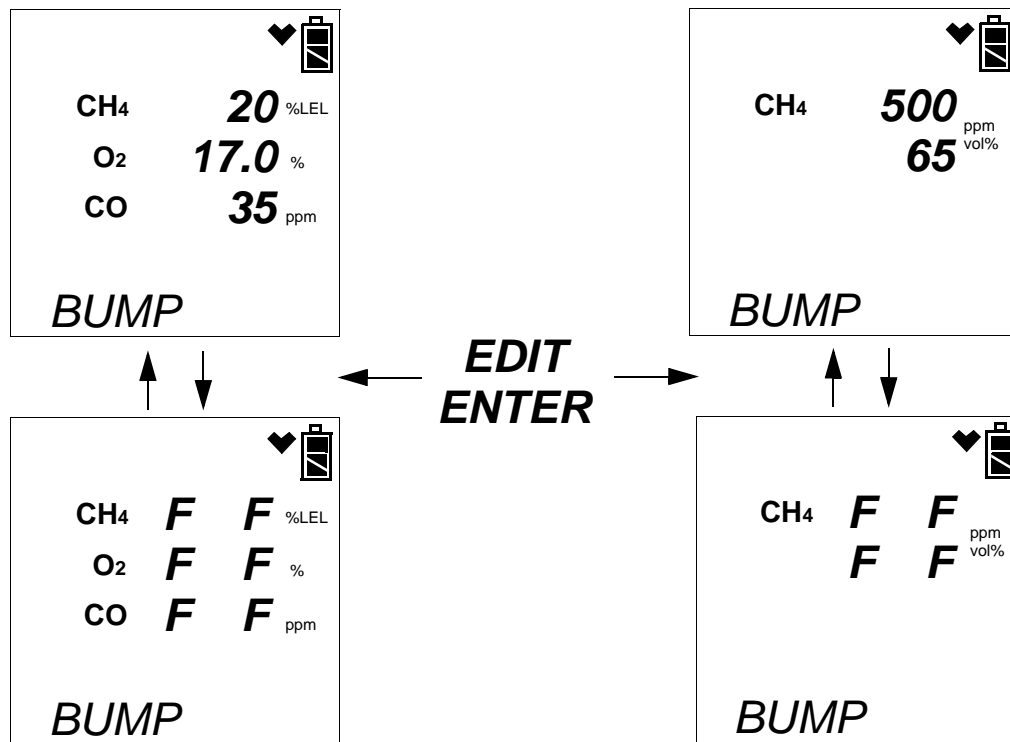
Figure 40: Failed Bump Test and Calibration, %Volume Sensor Installed and GAS Menu Item in Edit Mode Set to ALL
