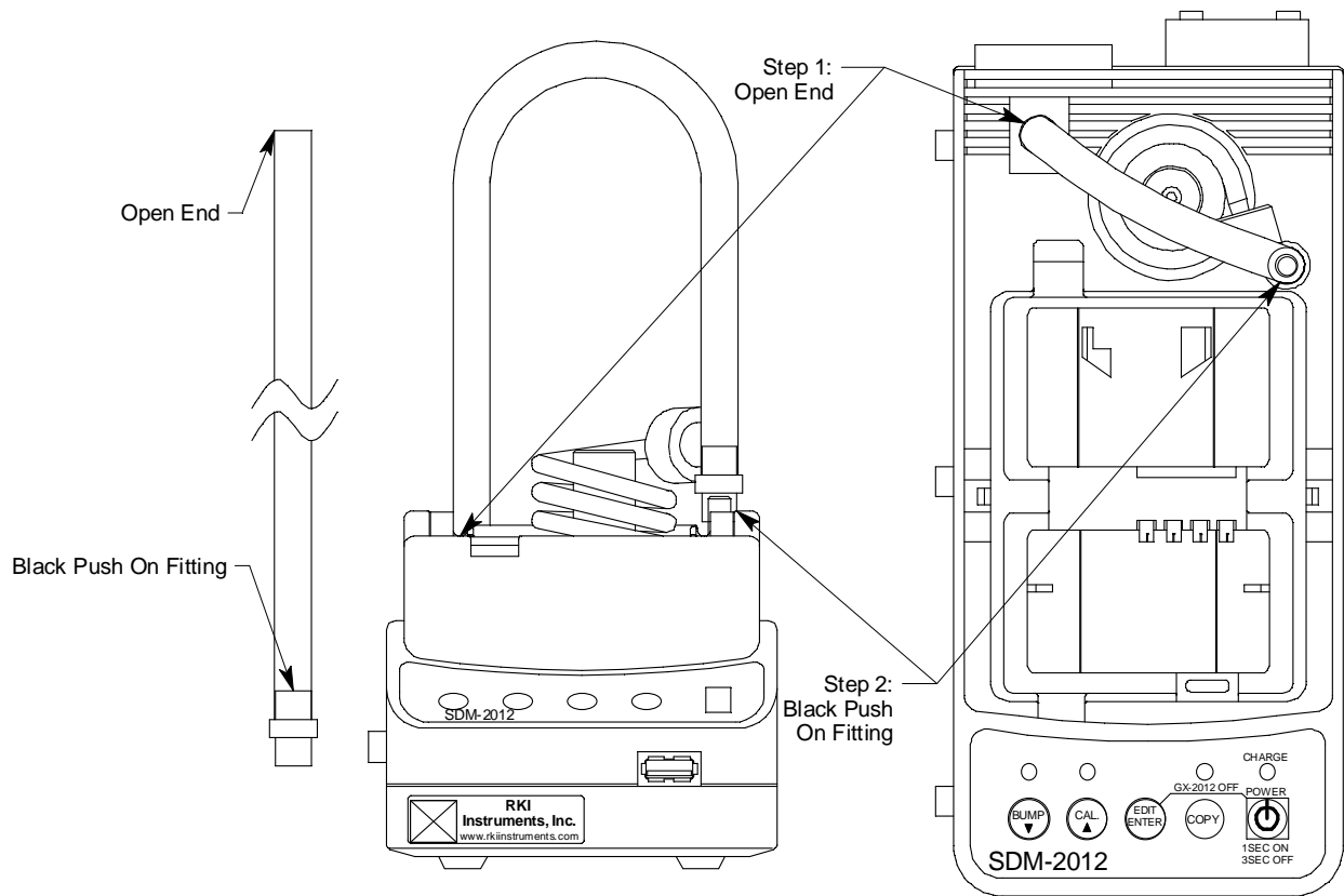
Figure 12: Installing the Exhaust Line
