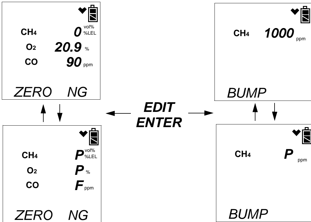
Figure 31: Fresh Air Adjustment Fail, Standard Gas Tracer and GAS Menu Item in Edit Mode Set to ALL
