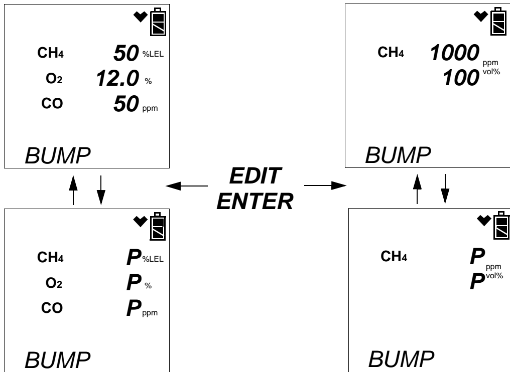
Figure 34: Successful Bump Test, %Volume Sensor Installed and GAS Menu Item in Edit Mode Set to ALL
