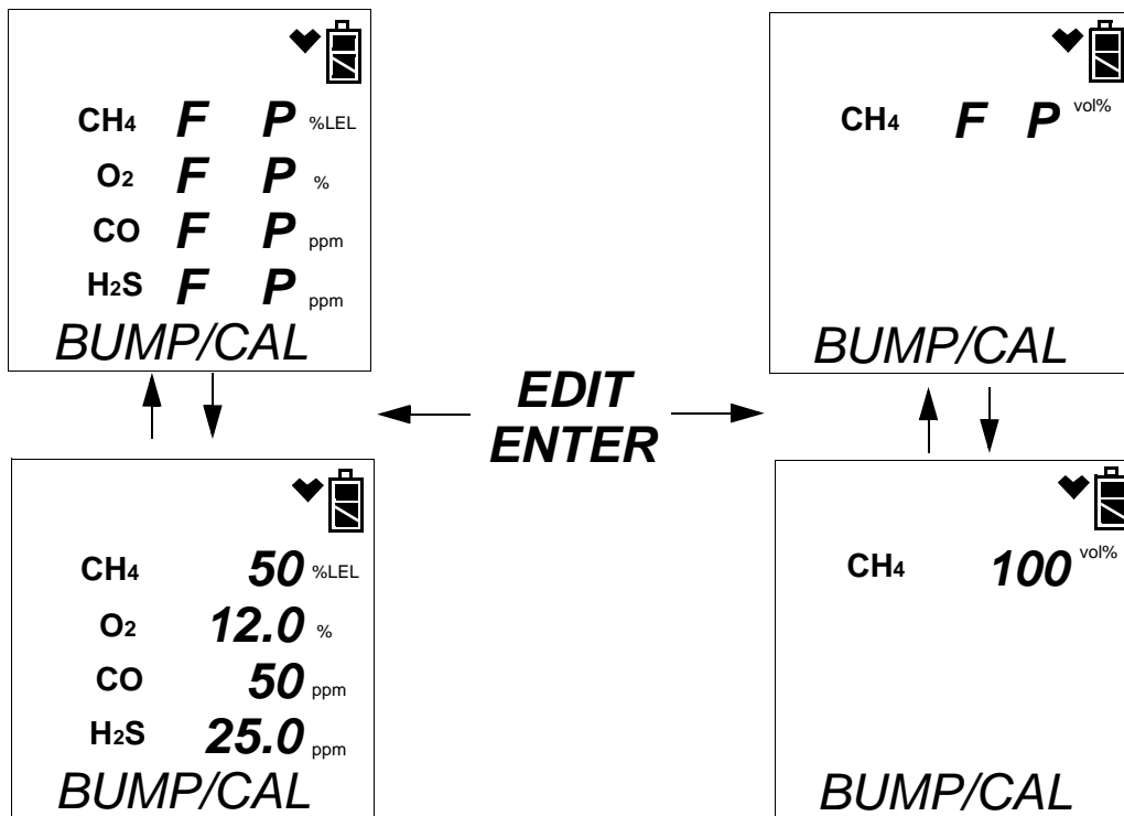
Figure 22: Screen Indication for Failed Bump Test and Passed Auto Calibration, %Volume Sensor Installed and GAS Menu Item in Edit Mode Set to ALL
