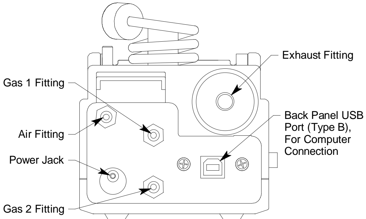
Figure 9: Fittings and Connections
