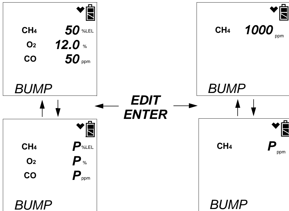
Figure 33: Successful Bump Test, Standard Gas Tracer and GAS Menu Item in Edit Mode Set to ALL
