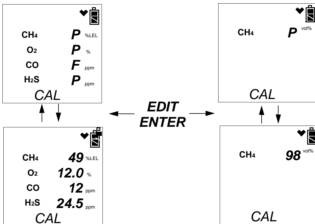
Figure 29: Calibration Results, %Volume Sensor Installed and GAS Menu Item in Edit Mode Set to ALL
