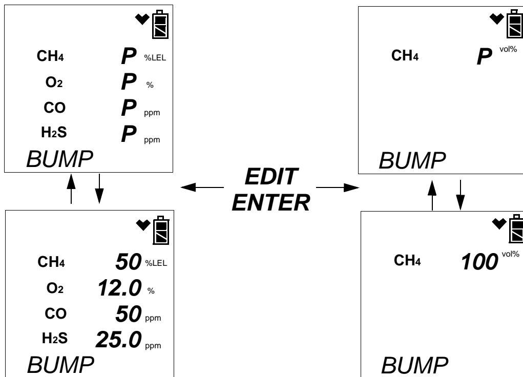
Figure 17: Screen Indication for Passed Bump Test, Standard 4-Gas GX-2012 or GAS Menu Item in Edit Mode Set to Std
