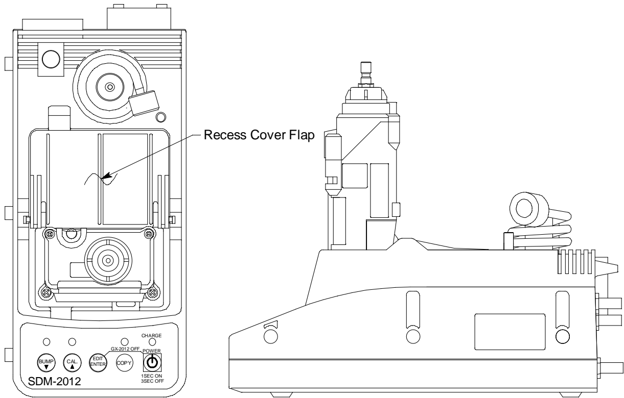
Figure 8: Instrument Panel with Lithium Ion Instrument Installed
