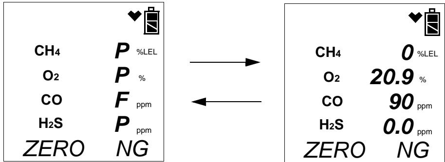
Figure 26: Failed Fresh Air Adjustment, Standard 4-Gas GX-2012 or GAS Menu Item in Edit Mode Set to Std
