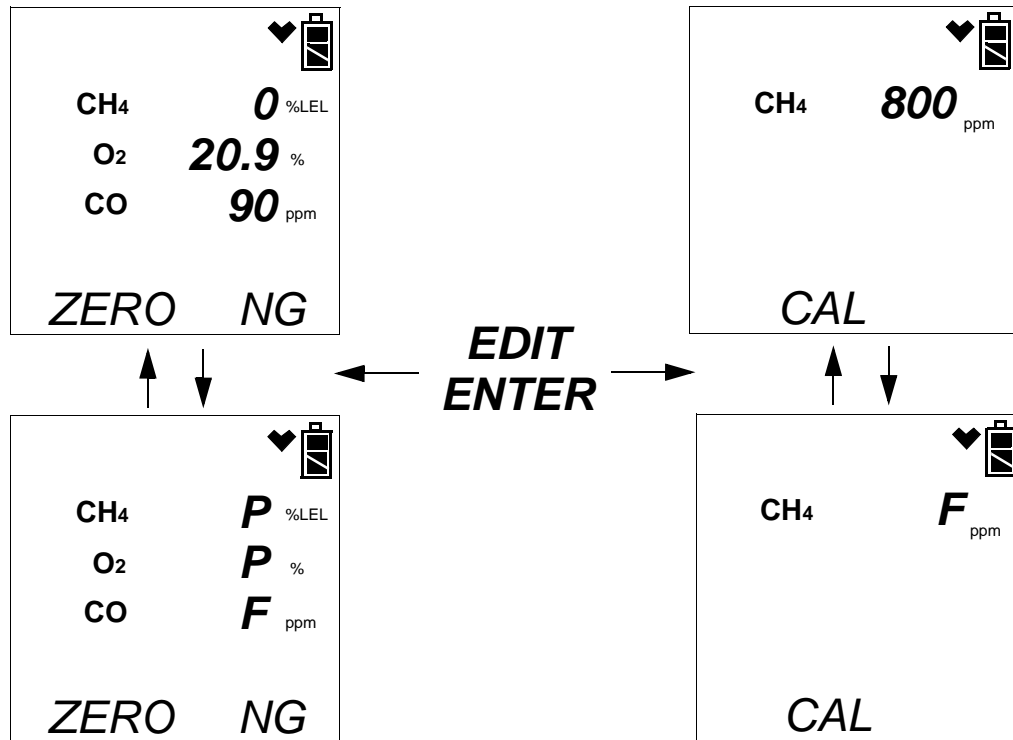
Figure 42: Failed Fresh Air Adjustment, Standard Gas Tracer and GAS Menu Item in Edit Mode Set to ALL
