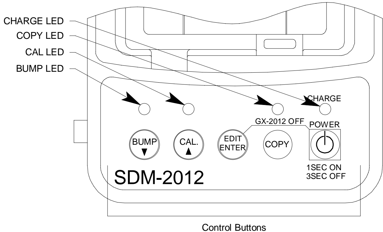
Figure 10: Control Panel
