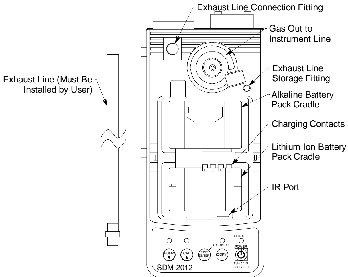
Figure 6: Instrument Panel (Shown Without Recess Cover Flap)
