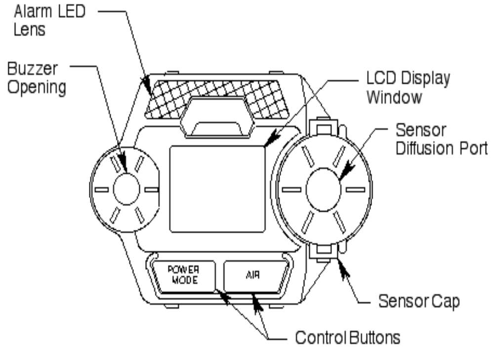
Figure 1 : Components of the GasWatch2
